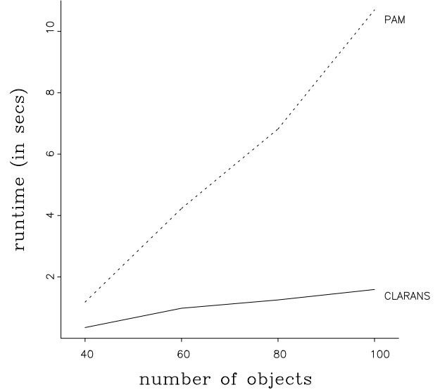
Figure 1: Efficiency: CLARANS vs PAM
